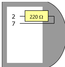
Figure 6; Terminating plug PIN assignment
